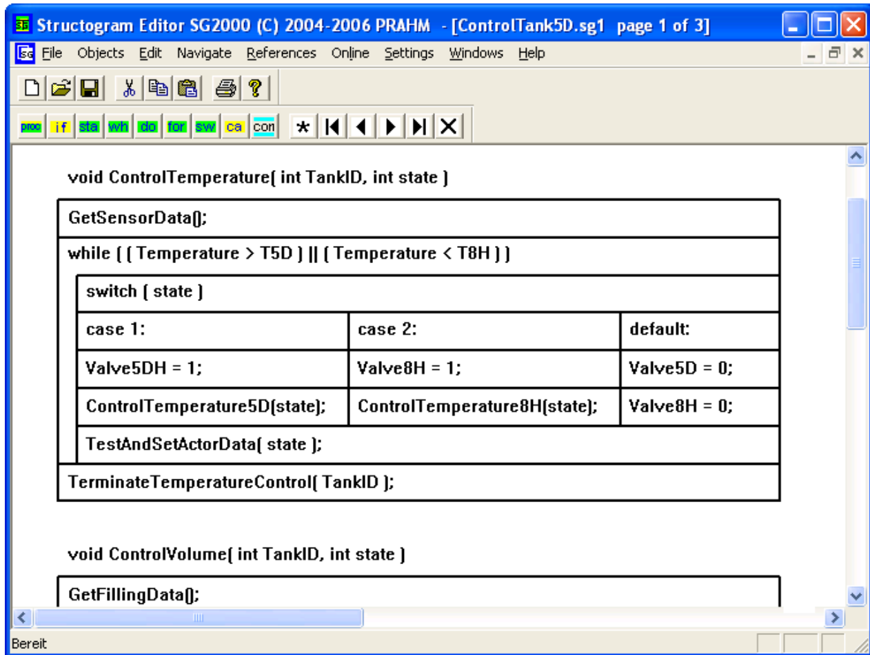
1 - The user interface of the PMS Structogram Editor
